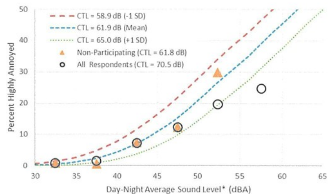
FIG. 3. (Color online) The percent Highly Annoyed for each sound level category represents the response of the population living near wind turbines in the U.S. (the data are weighted). Results are binned in 5 dB DNL* increments. The points for non-participating respondents exclude respondents who were compensated or hosted wind turbines on their property; the datasets diverge above the 45 to 50 dB sound level category. CTL curves for 58.9 and 65 dB are the \pm 1 SD exposure response for wind turbine noise as reported in Michaud et al. (2016b).
