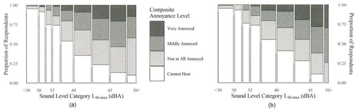
FIG. 2. Composite annoyance: distribution of outdoor audibility and annoyance level by sound level category for (a) all respondents ( n = 747 ; two respondents who indicated wind turbine audibility but did not provide an annoyance level are excluded from the plot) and (b) for only non-participants ( n = 591 ; two respondents who indicated wind turbine audibility but did not provide an annoyance level are excluded from the plot). Bar widths are proportional to the number of respondents in each exposure category. Each bar represents a grouping of 2.5 dBA, except for the top sound level category, which includes respondents with modeled sound levels greater than or equal to 47.5 dBA.
